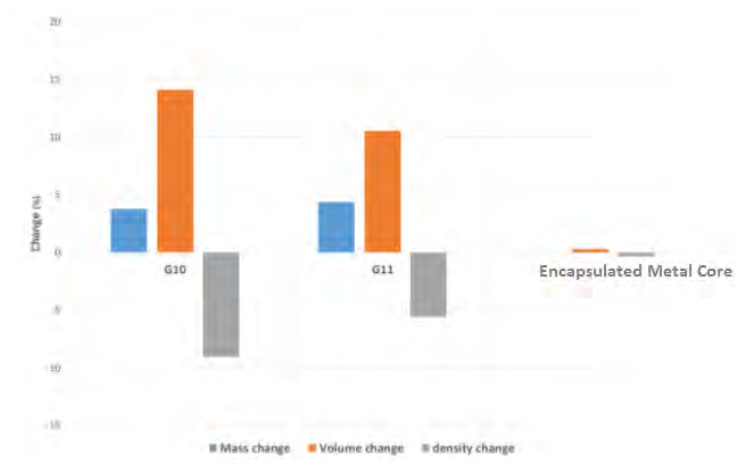
Figure 20: Mass/Volume/Density Change After Exposure
