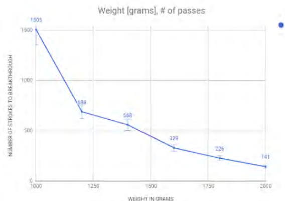
Figure 25: Taber Abrasion Test Results
