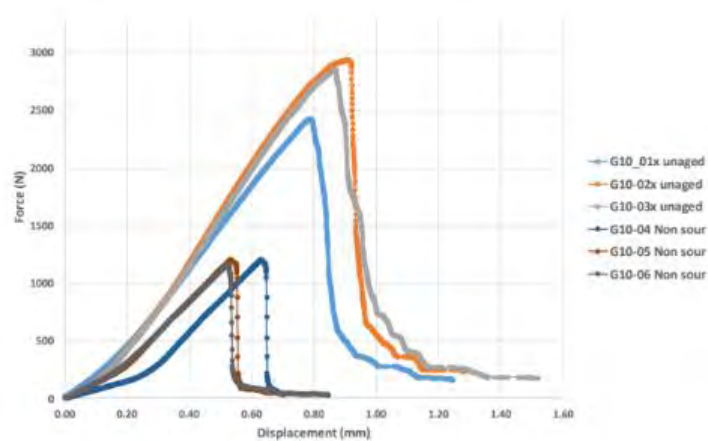
Figure 22: Force- displacement curves for G11 control specimens, and samples exposed in sour fluid at 150°C
